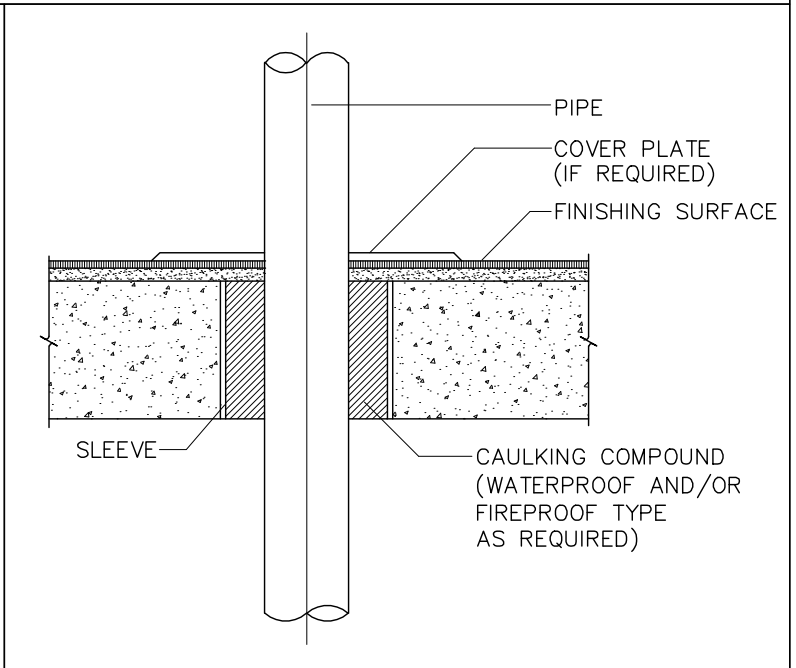
PIPE THROUGH FLOOR NOT TO SCALE
