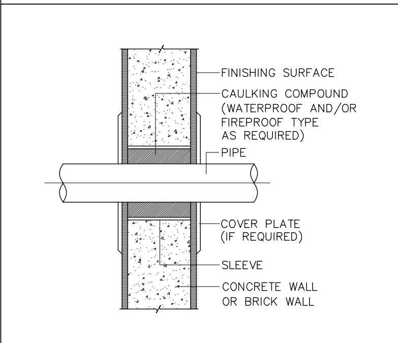
PIPE THROUGH WALL NOT TO SCALE
