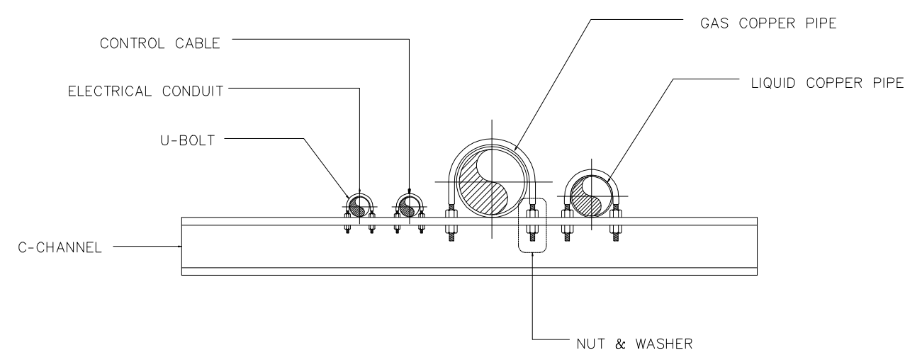
DETAIL PIPING
