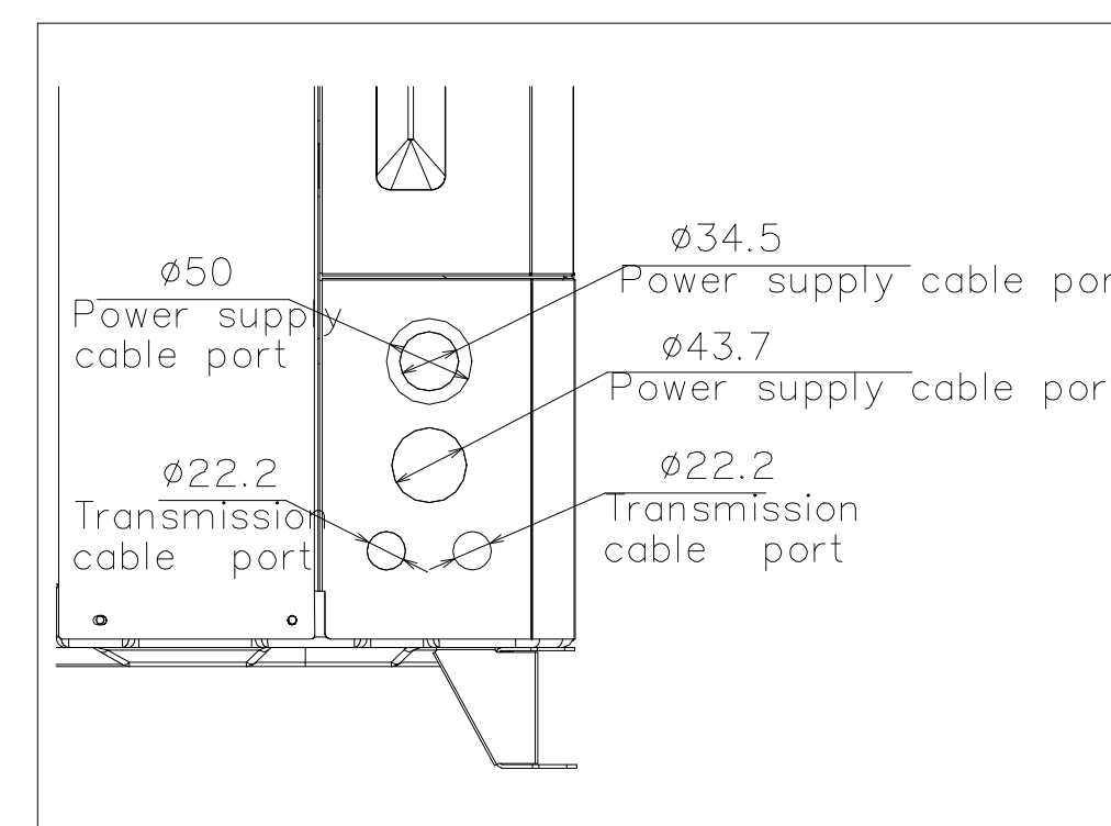
Detail B : Left view
