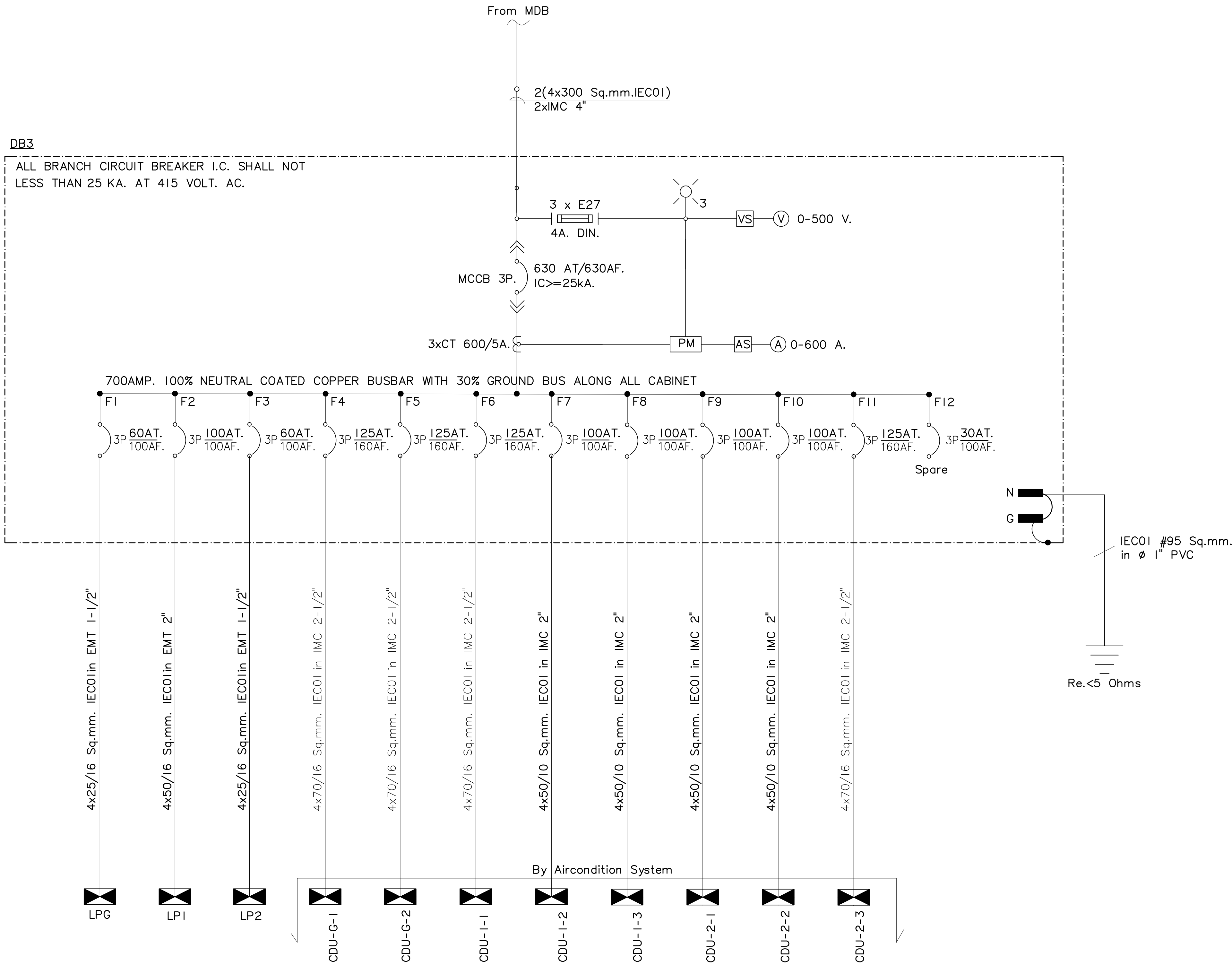
ELECTRICAL SYSTEM SINGLE LINE DIAGRAM
