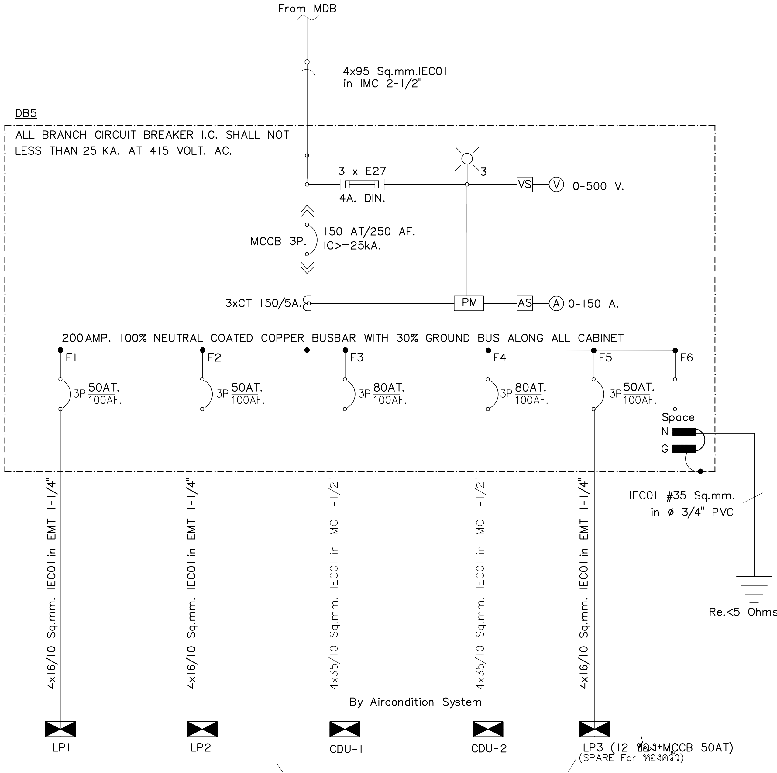
ELECTRICAL SYSTEM SINGLE LINE DIAGRAM
