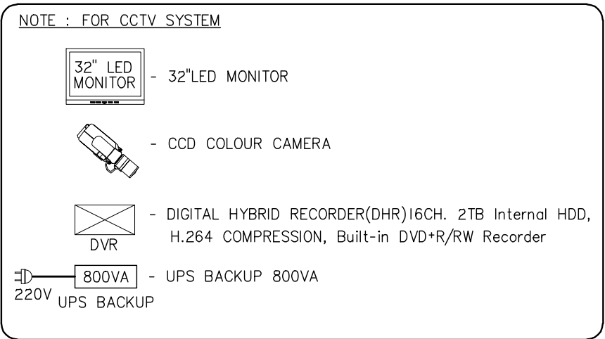
RISER DIAGRAM CCTV SYSTEM
