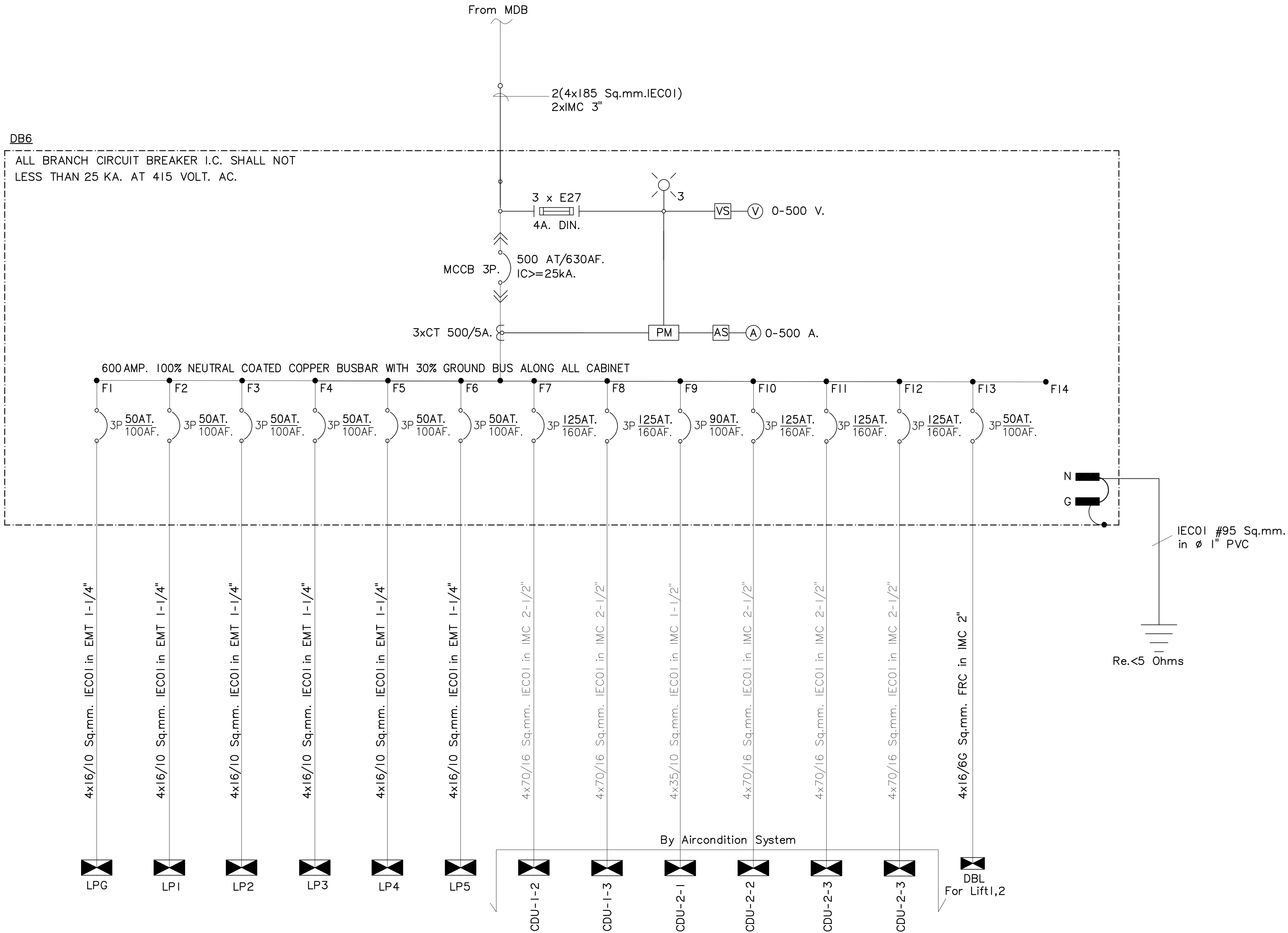
ELECTRICAL SYSTEM SINGLE LINE DIAGRAM
