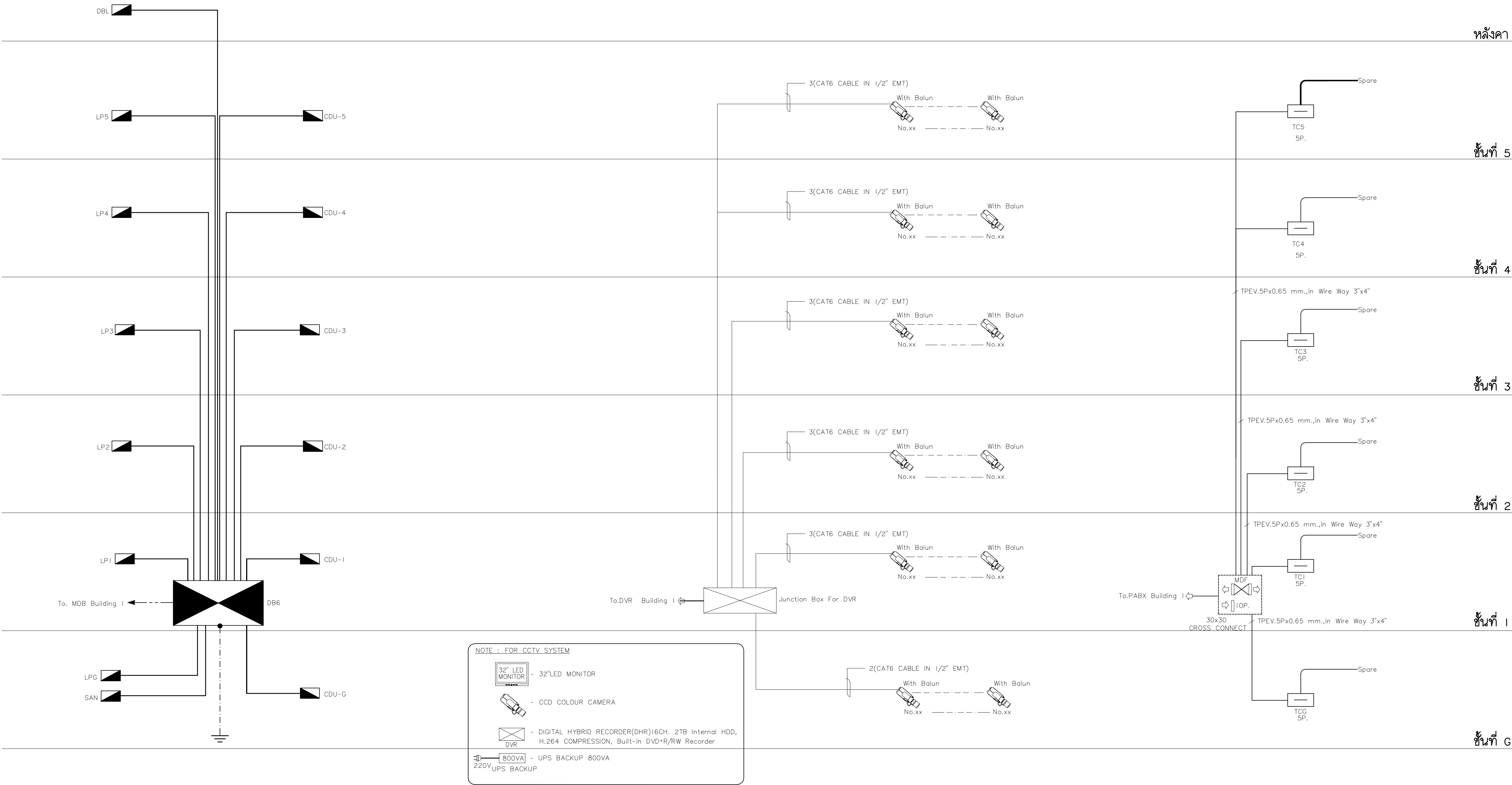
ELECTRICAL SYSTEM RISER DIAGRAM
