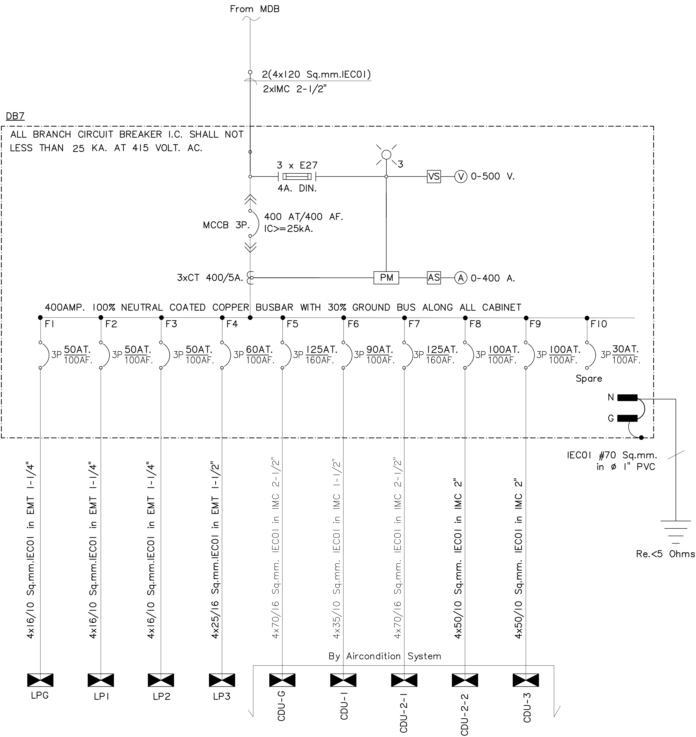
ELECTRICAL SYSTEM SINGLE LINE DIAGRAM
