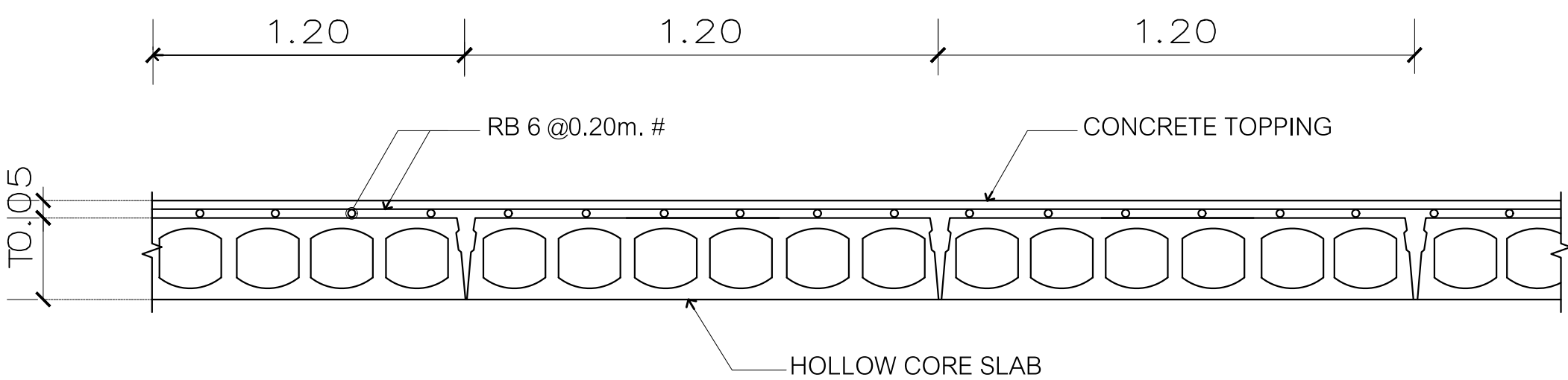
TYPICAL CROSS SECTION OF HOLLOW CORE SLAB
