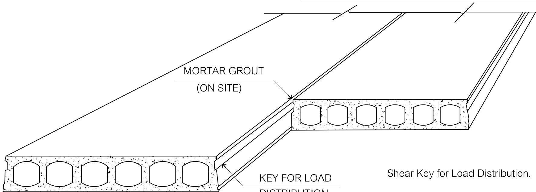
Shear Key for Load Distribution.
