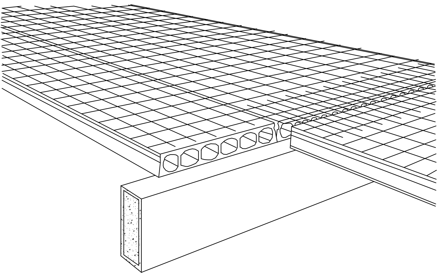
Hollow Core Slab on RC Beam.
