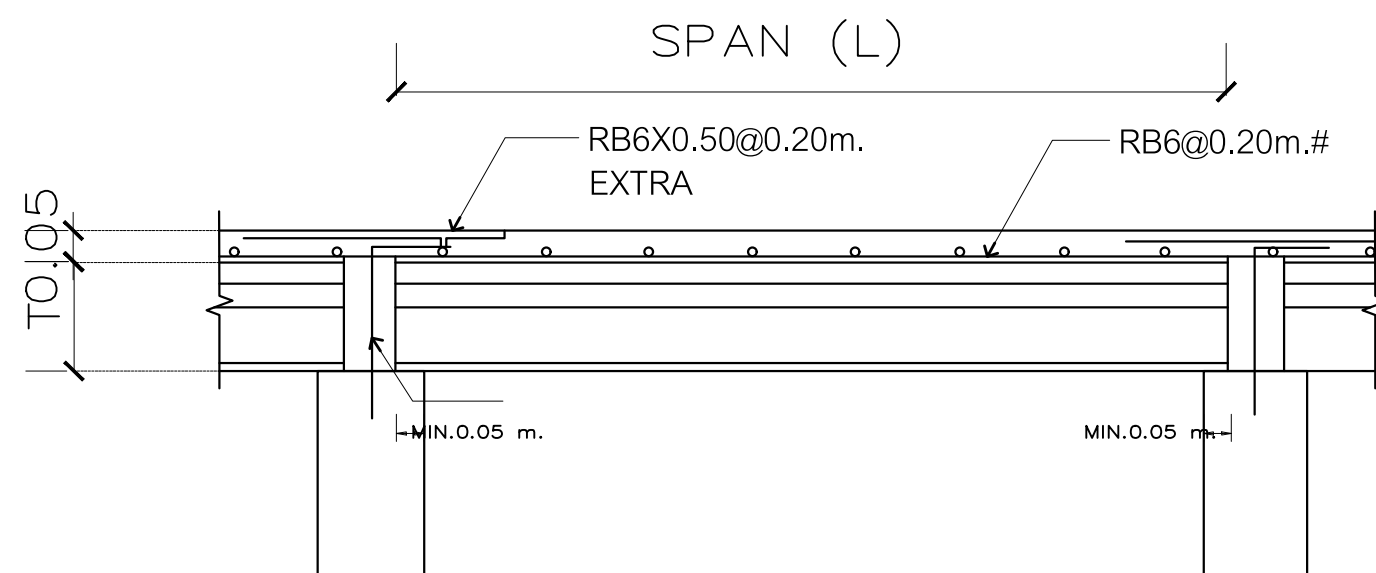
TYPICAL LONGITUDINAL SECTION T= 1:20
