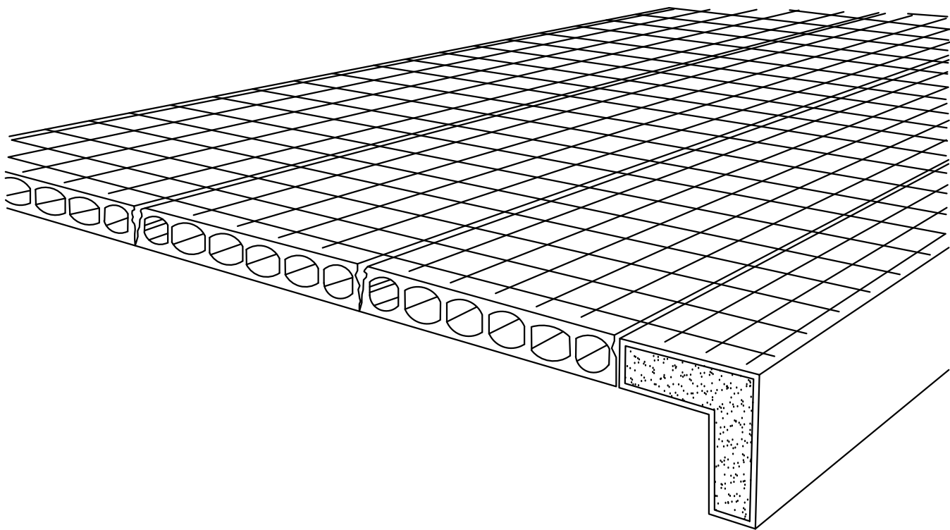
Hollow Core Slab on RC Beam.
