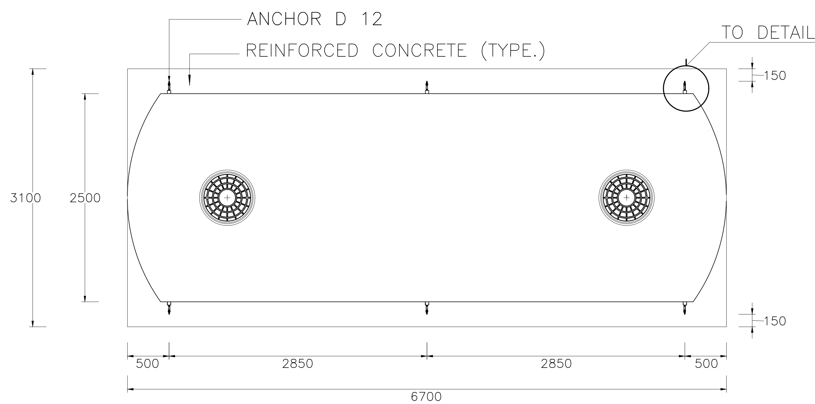
PLAN-TOP SLAB REINFORCEMENT
