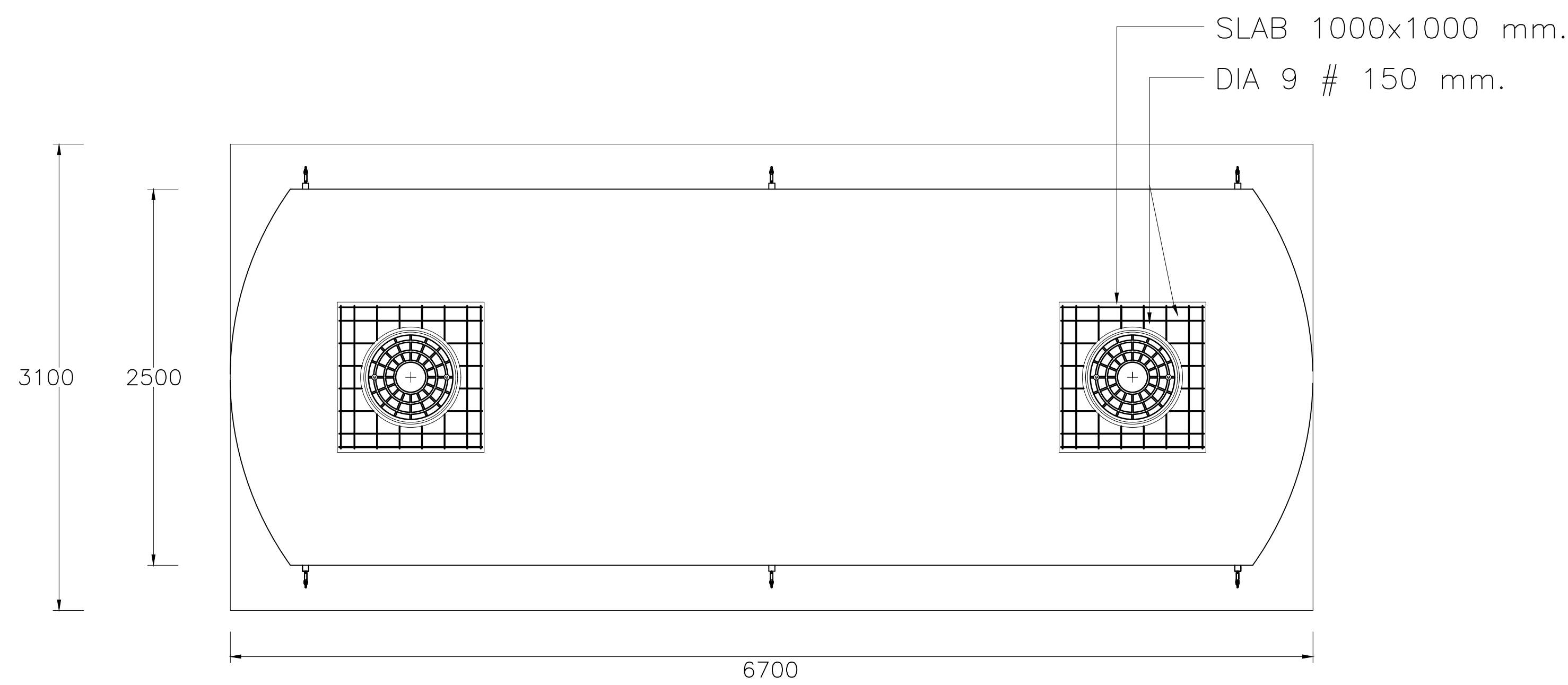
PLAN-TOP SLAB REINFORCEMENT
