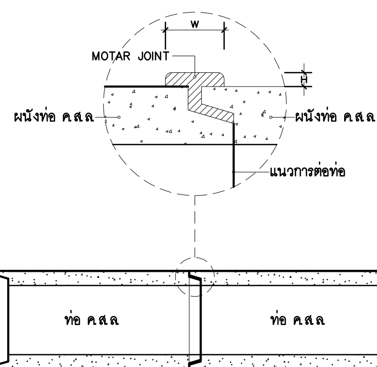
DETAIL OF REINFORCE CONCRETE PIPE
