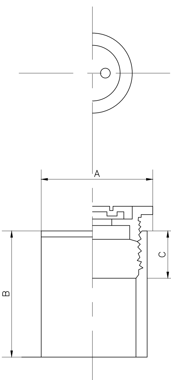
FLOOR CLEANOUT P.V.C.
