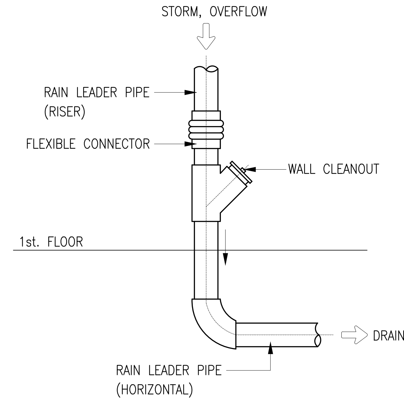
DRAIN PIPE INSTALLATION
