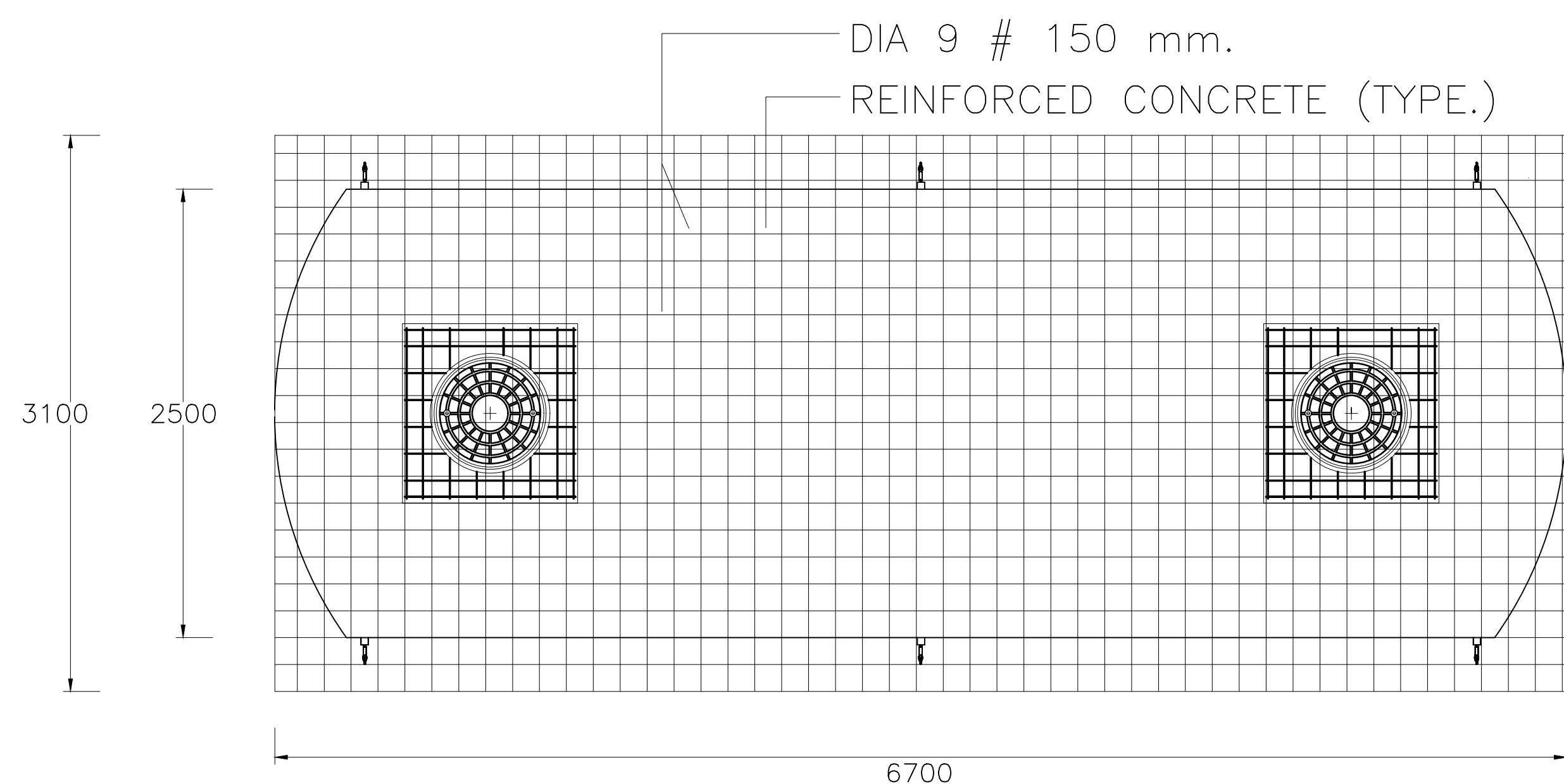
PLAN-BASE SLAB REINFORCEMENT
