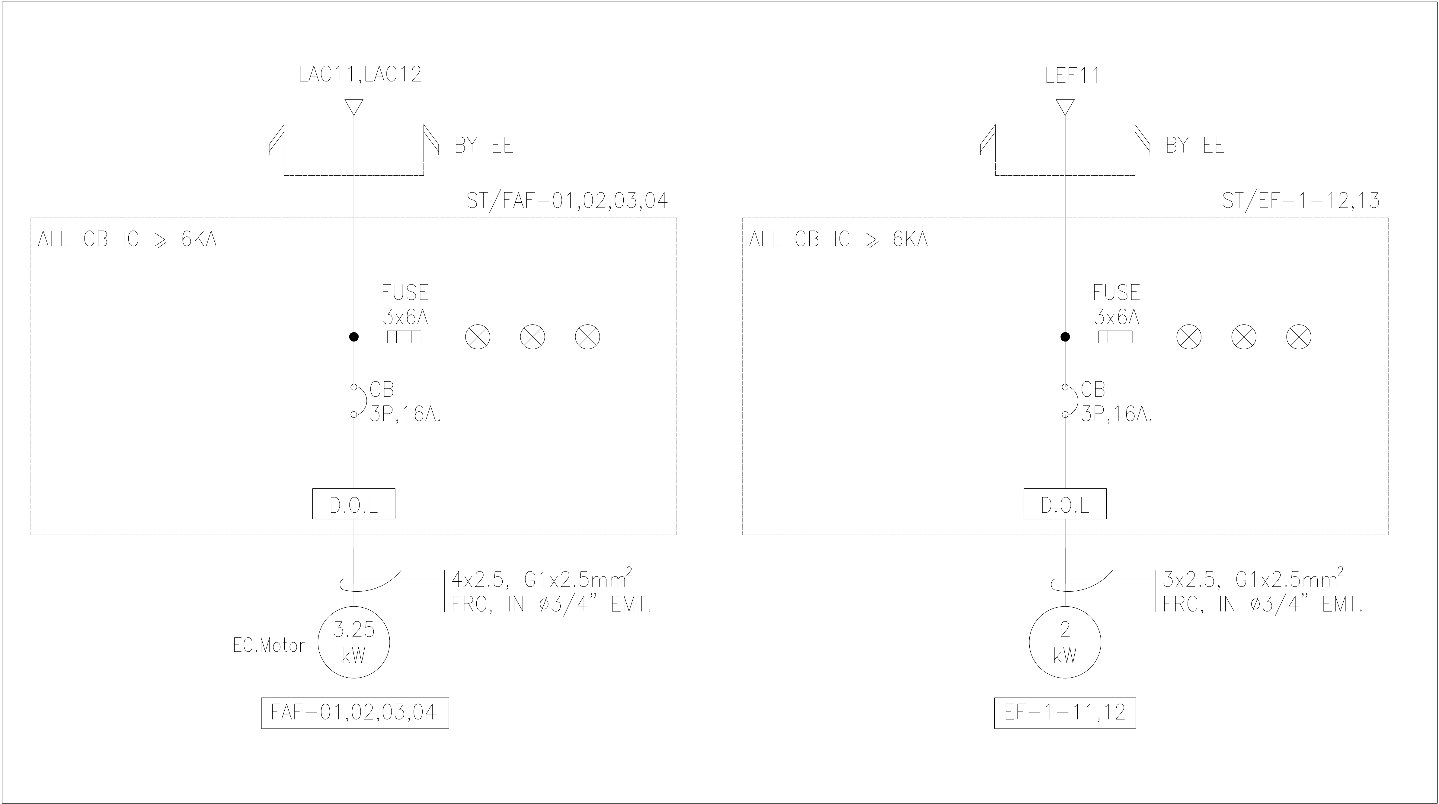
03 ELECTRICAL DIAGRAM FOR EXHAUST FAN
